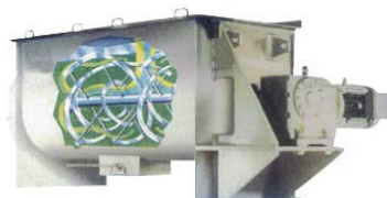
Ribbon mixer
