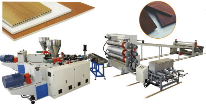
Wood Plastic Composite Sheet Extrusion Equipment
